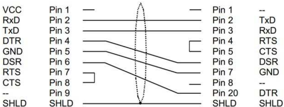
Printer (DSUB25 male)
